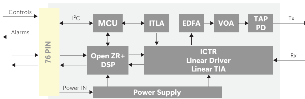
QSFPDD-400G-XZRP+ Block Diagram
